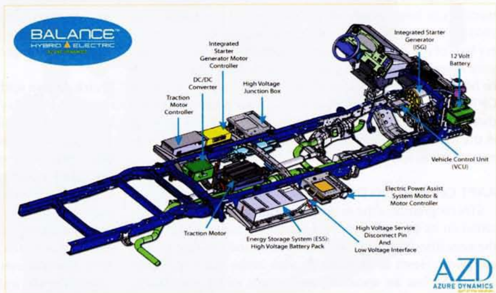
A schematic of the Azure Dynamics hybrid electric chassis for the Ford E-450 that Collins Bus Corporation will use in its Type As.
